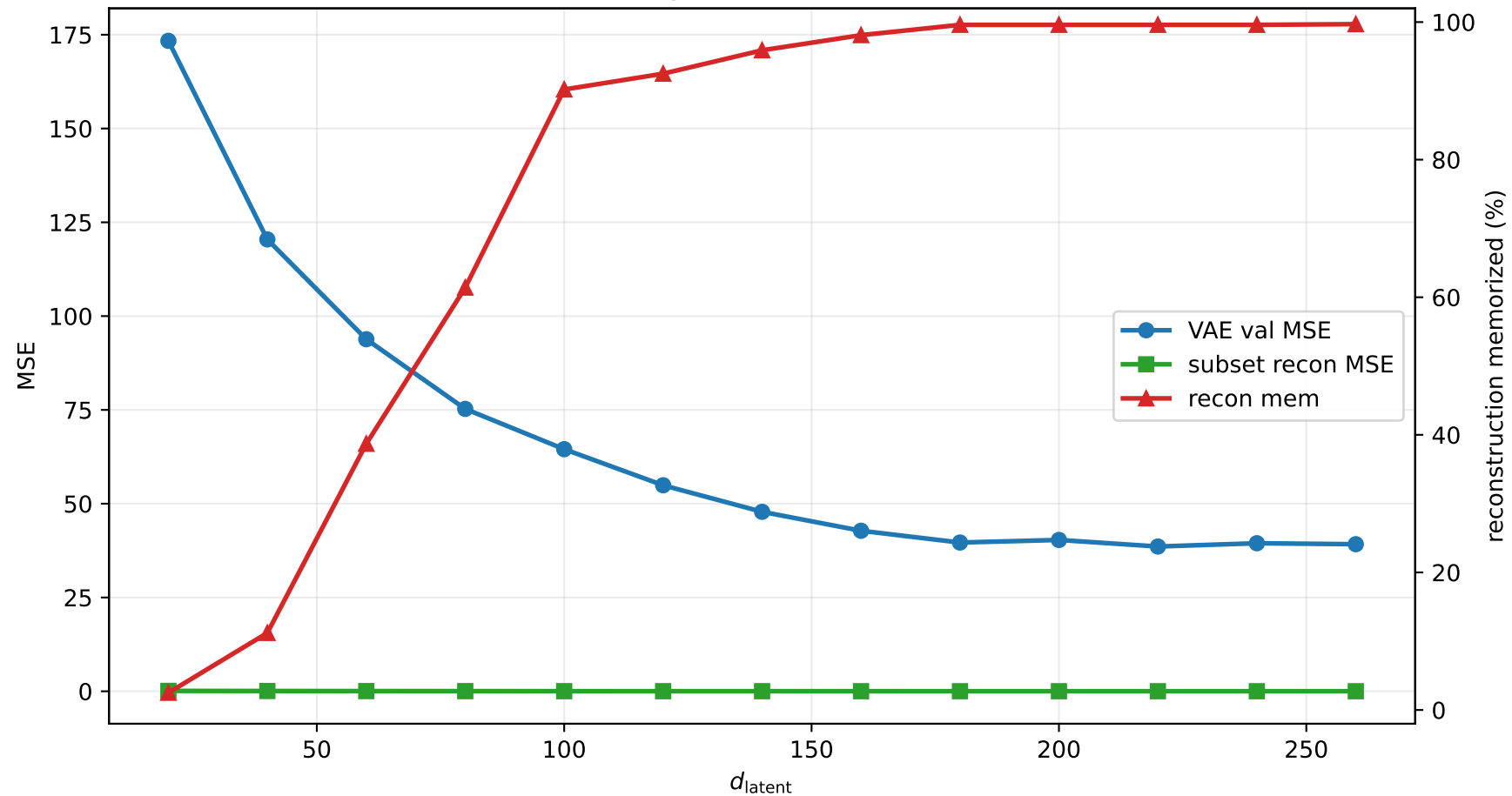
CIFAR-10: VAE Quality vs Reconstruction Memorization
